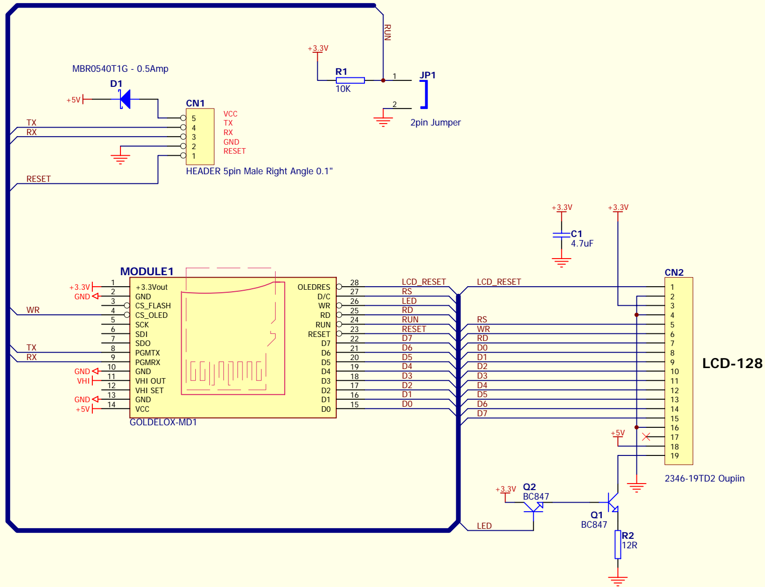
uLCD-128-GMD1 powered by GOLDELOX-MD1
